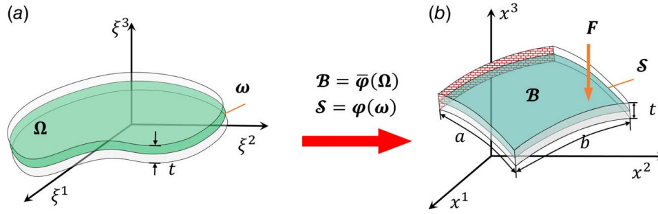
Fig. 6 Minimizing the compliance of a shell structure by topology optimization: (a) parametric domain and (b) physical domain
