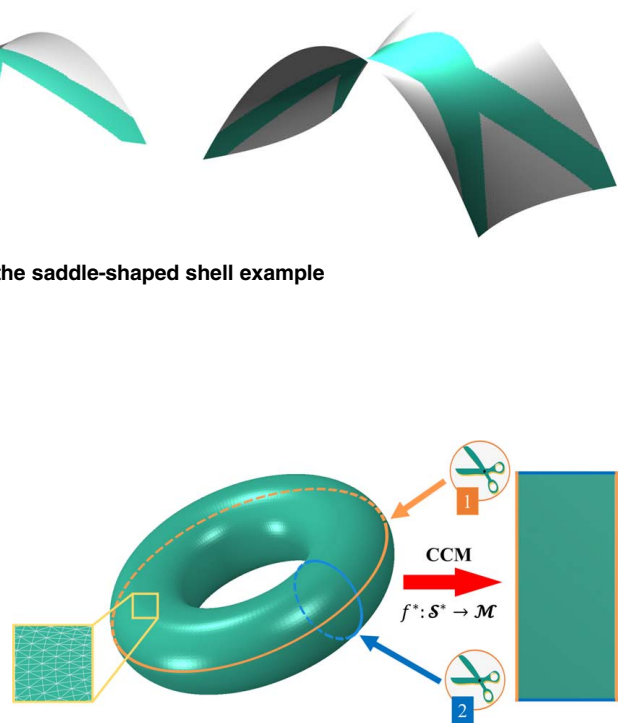
Fig. 13 Torus surface parameterization via cutting operation
