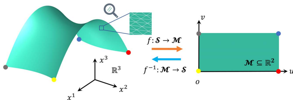
Fig. 8 Parameterization of the mid-surface of the saddle-shaped shell by computational conformal mapping
