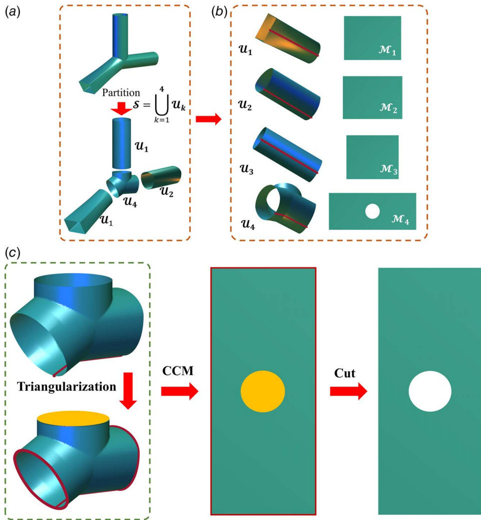
Fig. 18 Surface parameterization via multipatch stitching approach: (a) partition the surface into four patches, (b) surface parameterization of each patch, and (c) delaunay triangularization and parameterization
